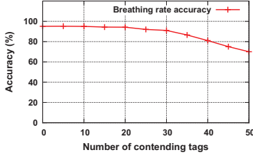
Figure 14. Breathing rate accuracy with different number of contending tags.
