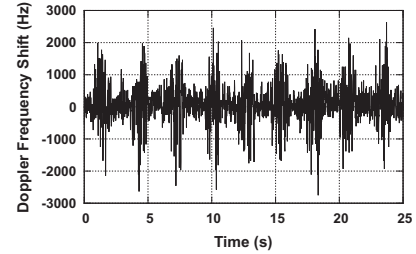
Figure 3. Raw Doppler frequency shift during the measurements.
