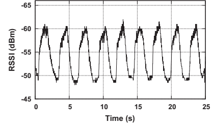
Figure 2. Raw RSSI readings during the measurements.
