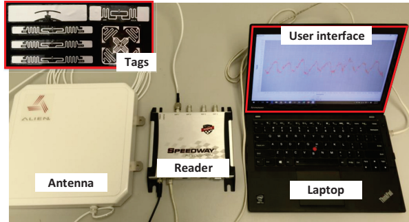
Figure 11. TagBreathe prototype system.
