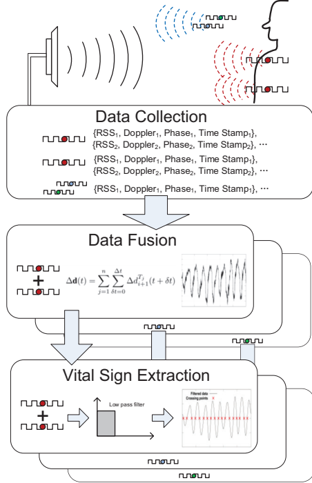
Figure 10. Illustration of TagBreathe workflow.
