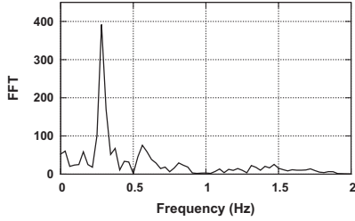
Figure 7. FFT for displacement values collected during the measurements.
