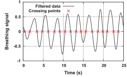
Figure 8. Extracted breathing signal from the measurements.
