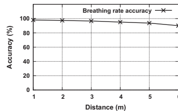
Figure 12. Breathing rate accuracy at different distances.
